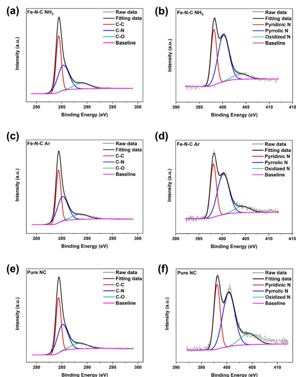
Fig. 4 High-resolution C 1s XPS spectra of Fe-N-C \text{NH}_3 (a), Fe-N-C Ar (c) and pure NC (e), respectively. High-resolution N 1s XPS spectra of Fe-N-C \text{NH}_3 (b), Fe-N-C Ar (d) and pure NC (f), respectively.
