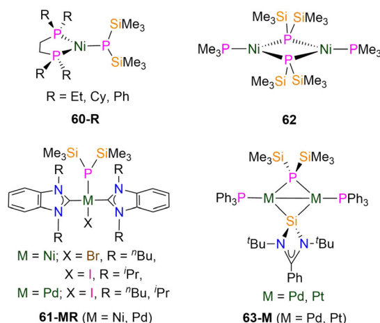
Fig. 18 Group 10 \text{P}'' complexes [\text{Ni}(\kappa^2\text{-drpe})(\text{P}'')] ( 60-R ; \text{drpe} = \text{R}_2\text{PCH}_2\text{CH}_2\text{PR}_2 , R = Et, Cy, Ph), [\text{M}(\text{X})(\text{R}_2\text{-bimy})_2(\text{P}'')] ( 61-MR , M = Ni, X = Br, R = n Bu, 61-Ni n Bu ; M = Ni, X = I, R = i Pr, 61-Ni i Pr ; M = Pd, X = I, R = n Bu, 61-Pd n Bu ; i Pr, 61-Pd i Pr ; bimy = benzimidazole-2-ylidene), [\text{Ni}(\text{PMe}_3)(\mu\text{-P}'')]_2 ( 62 ), \{[\text{M}(\text{PPh}_3)_2(\text{P}'')](\text{Si}(\text{N}^t\text{Bu})_2\text{CPh})\} ( 63-M ; M = Pd, Pt).
