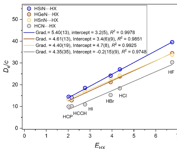
Fig. 8 Graphs of D_e/c versus E_{HX} for the four series HMN...HX (M = C, Si, Ge, Sn), (X = F, Cl, Br, I, CCH, CP) in which the atom M adjacent to that directly involved in the hydrogen bond belongs to Group 14.
