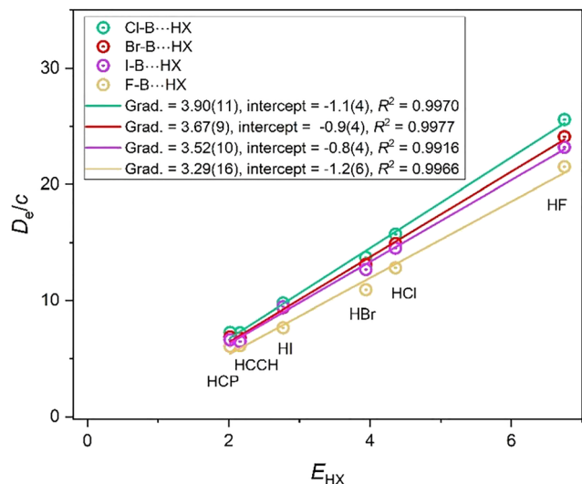
Fig. 6 Graphs of D_e/c for the four series MB...HX (M = F, Cl, Br, I, and X = F, Cl, Br, I, CCH, CP) in which the atom M adjacent to that directly involved in the hydrogen bond belongs to Group 17 of the periodic table.
