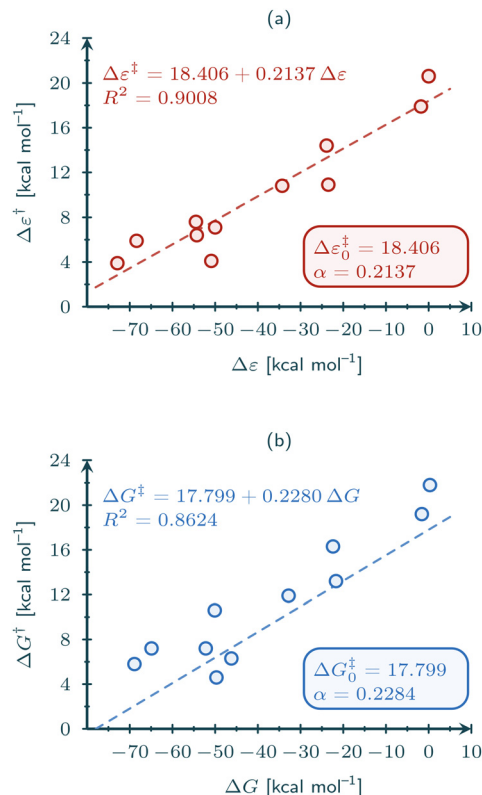
Fig. 3 Activation barrier as function of the reaction energy for the S N 2 reaction of chloromethane with different nucleophiles. Data are shown as (a) electronic energies ( ε ) and (b) Gibbs free energies ( G ).
