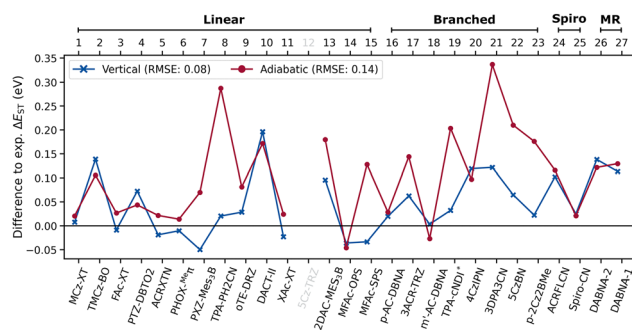
Fig. 3 Difference between experimental and computed \Delta E_{ST} as obtained with DFT/MRCI using the R2018 Hamiltonian, short settings and a B3LYP/def2-SVP anchor configuration. Vertical gaps were obtained using PBEh-3c S_0 gas phase geometries (blue crosses) whereas the ROKS/UKS OT-LC- \omega PBE-D3(BJ)/def2-SVP+PCM excited S_1 and T_1 geometries (dark red circles) were used to determine adiabatic gaps.
