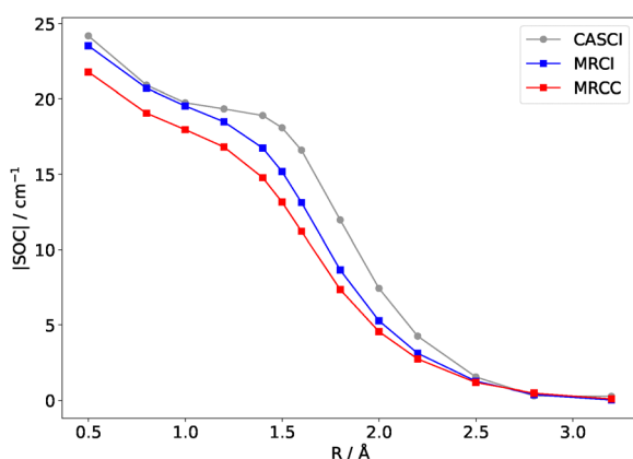
Fig. 1 Run of the computed spin–orbit coupling matrix elements between the X 3 Σ − and the c 1 Π state of NH. The computations use the cc-pCVDZ basis set, all electrons were correlated. For MRCC, the averaged value is plotted, see text.
