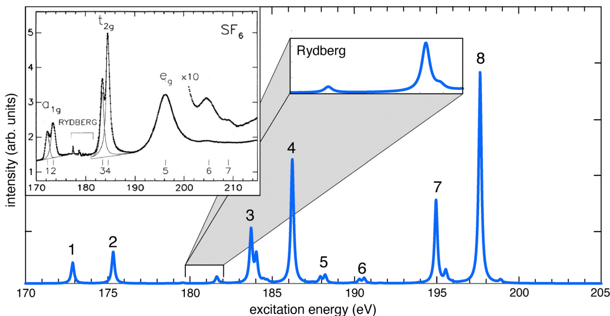
Fig. 7 L-edge XAS of \text{SF}_6 . The CAM-B3LYP/CIS + SOC spectrum (in blue) was obtained using the def2-TZVPPD basis set with 200 singlet and 200 triplet states. Individual transition energies were shifted by 5 eV and broadened with a Lorentzian function (FWHM = 0.3 eV). The experimental spectrum (inset) is reproduced from ref. 134; copyright 1993 American Physical Society.
