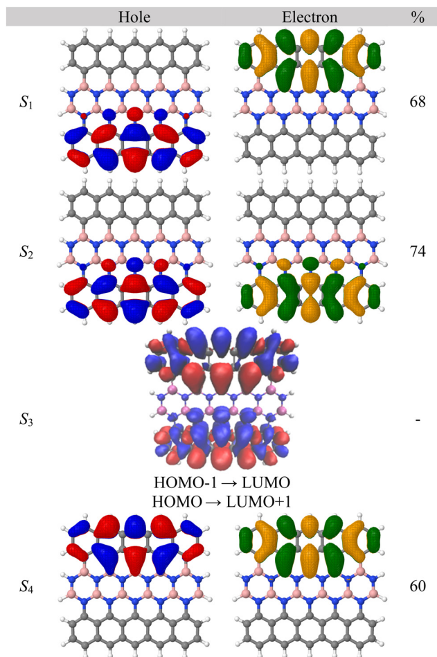
Fig. 6 BN-center NTOs obtained at the MR-CISD level of theory, for the transition to the S_1 , S_2 and S_4 states. (isovalue \pm 0.04 e bohr ^{-3} ). S_3 state consists of a double excitation ( \text{HOMO}-1 \rightarrow \text{LUMO} , \text{HOMO} \rightarrow \text{LUMO}+1 ), the density difference between this state and S_0 was plotted in this case (isovalue of \pm 0.0005 e bohr ^{-3} ) and the red color means a decrease in electron density, while blue indicates that the density increased.
