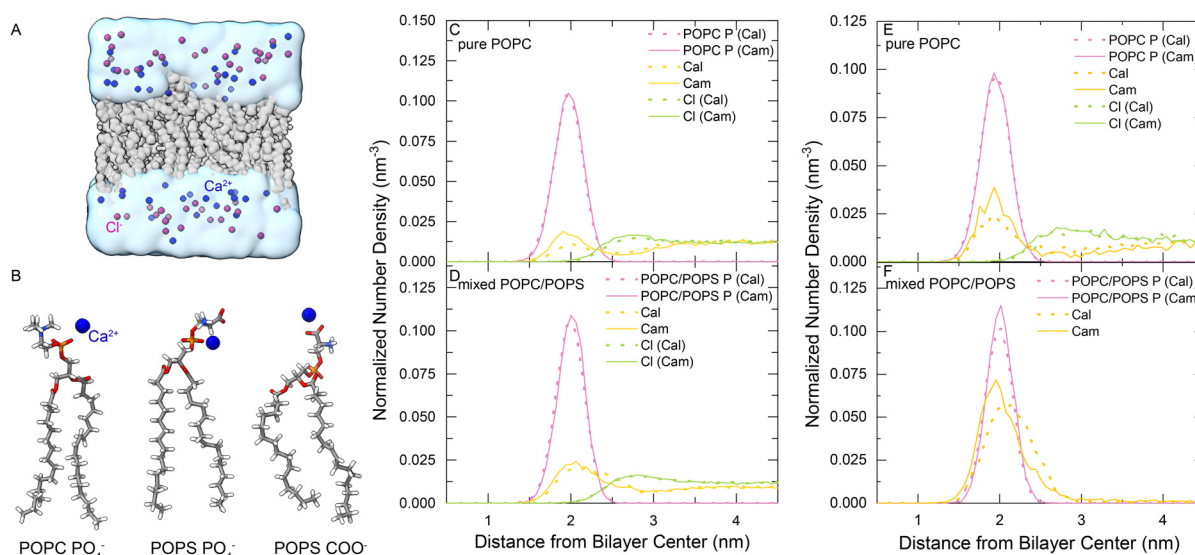
Fig. 1 (A) Single-membrane simulation system. The lipid bilayer is shown in gray. \text{Ca}^{2+} and \text{Cl}^{-} ions are shown in blue and purple, respectively. Water is shown with a transparent cyan surface. (B) Representative structures of the \text{Ca}^{2+} -lipid complexes. A \text{Ca}^{2+} ion was bound to the \text{PO}_4^{-} of POPC, \text{PO}_4^{-} of POPS, and \text{COO}^{-} of POPS. (C) and (D) Density profiles of selected groups calculated along the bilayer normal direction for pure POPC or mixed POPC/POPS bilayers with 1 M \text{CaCl}_2 . (E) and (F) Density profiles of selected groups calculated along the bilayer normal direction for pure POPC or mixed POPC/POPS bilayers with 200 mM \text{CaCl}_2 . The solid lines were obtained using the multisite \text{Ca}^{2+} model ( Cam ) and the dashed lines were obtained using the default \text{Ca}^{2+} model ( Cal ).
