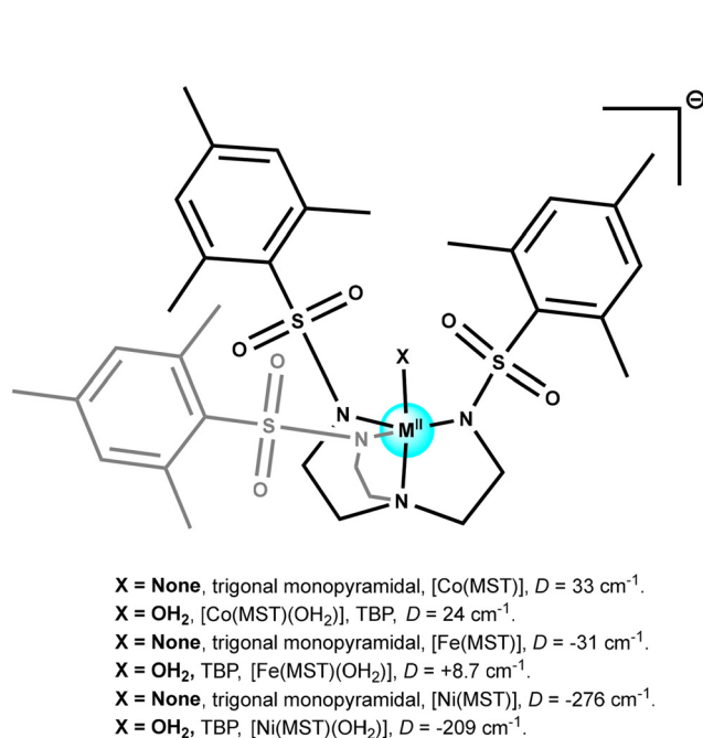
Fig. 17 Schematic representation of complexes 19 and 19' (left); CASSCF-computed principal magnetic anisotropy axes ( D_{xx} , D_{yy} , and D_{zz} ) are shown as pink dotted lines for the cobalt complex (a, 19a and b, 19a' ). The blue arrow highlights the direction and orientation of the D_{zz} , while the green arrows represent the molecular orientation axes (right), 94 adapted/reproduced from ref. 94 with permission from The Royal Society of Chemistry, 94 copyright 2018.
