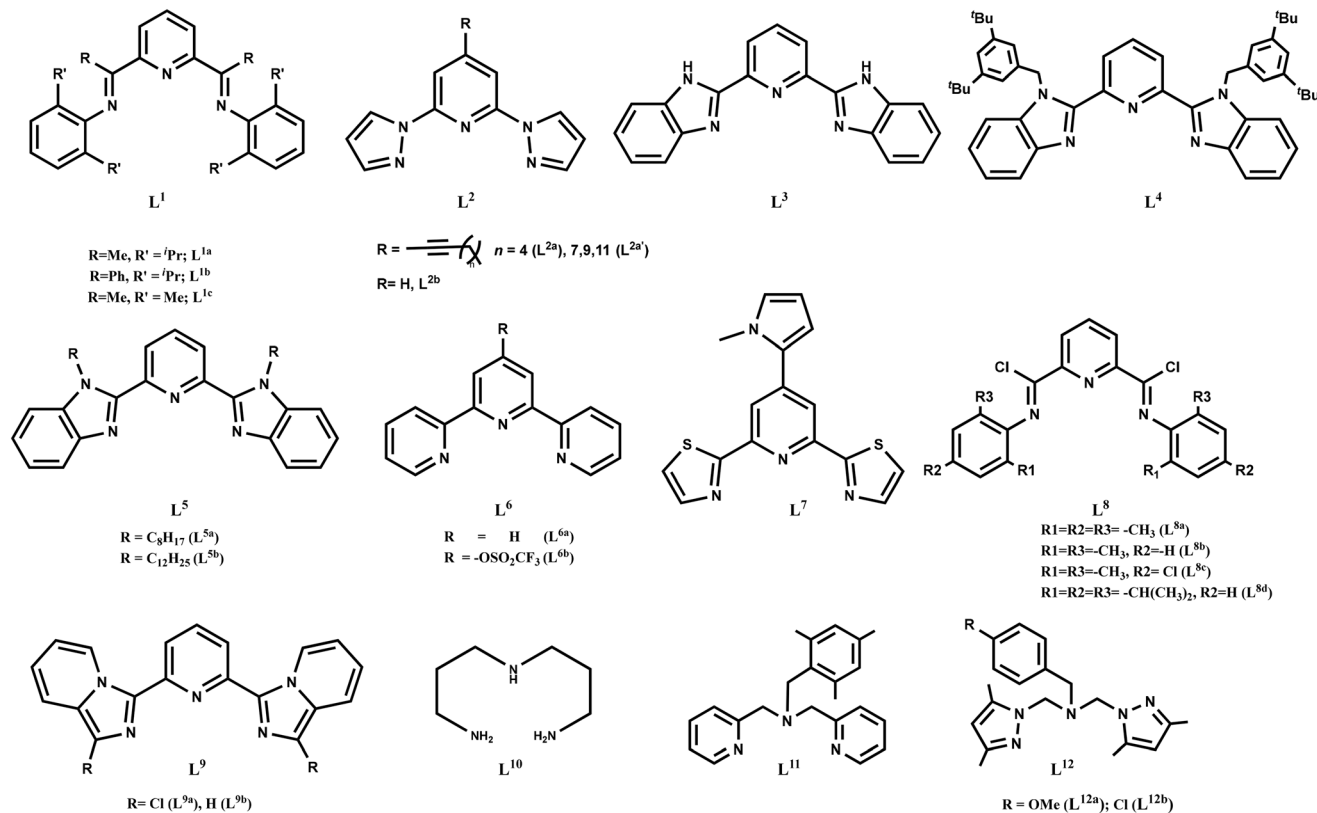
Chart 1 The ligands used to construct the Co II NNNX 2 -based SIMs mentioned in Table 1.
