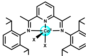
X = SeCN; Sq. Pyramidal, d = 0.39 \text{ \AA} , D = -53.4 \text{ cm}^{-1} . X = Cl; Sq. Pyramidal, d = 0.55 \text{ \AA} , D = -55.4 \text{ cm}^{-1} . X = Br; Sq. Pyramidal, d = 0.54 \text{ \AA} , D = -32.1 \text{ cm}^{-1} .
