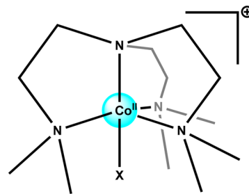
X = Cl, TBP, D = -6.2 cm -1 X = Br, TBP, D = -7.9 cm -1
