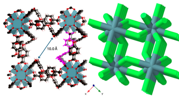
Fig. 3 [\text{Zr}_6(\text{bttb})_4(\text{O})_4(\text{OH})_4] CTH-42 with one \text{bttb} linker in pink, and the 3,12-c lj net describing the structure. The narrowest diameter of the channels in z-direction is given.
