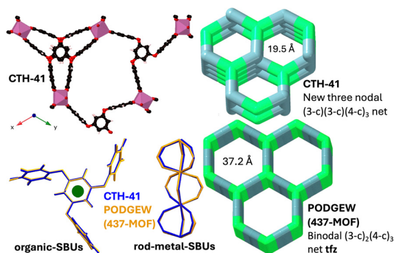
Fig. 2 Left: Crystal structure of [\text{In}_3(\text{bttb})_2(\text{OH})_3] CTH-41 , and superposition of the organic SBUs and metal-SBUs of [\text{In}_3(\text{bttb})_2(\text{OH})_3] CTH-41 , and [\text{In}_3(\text{bttb})_2(\text{OH})_3] 437-MOF . Right: The nets in [\text{In}_3(\text{bttb})_2(\text{OH})_3] CTH-41 , and [\text{In}_3(\text{bttb})_2(\text{OH})_3] 437-MOF using the STR approach. The largest rings in the CTH-41 net is 8 whereas in tfz it is 10 nodes.
