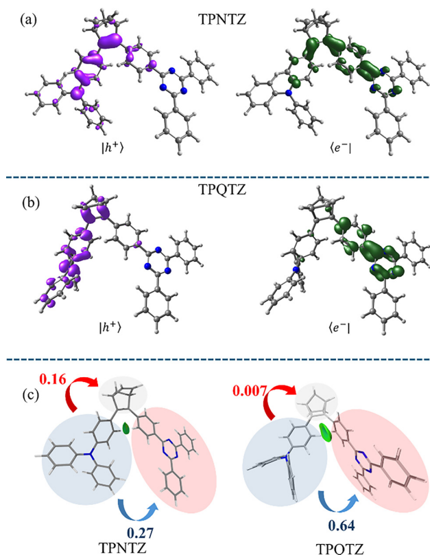
Fig. 3 (a) Hole–electron analysis (NTOs: |h^+ \rangle , violet; |e^- \rangle , green) for transition corresponding to the S1 and T1 excited states of (a) TPNTZ and (b) TPQTZ at isosurface values of \pm 0.002 a.u. [M06-2X/6-31g(d,p)]. (c) 3D visualization of non-covalent interaction and charge transfer amount in TPNTZ and TPQTZ (left to right); green isosurface refers to interactions.
