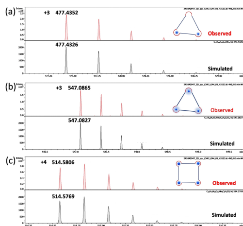
Fig. 2 The observed and simulated peaks found in the S-CM-2 and T-CM-2 mixtures. (a) [\text{C}_{78}\text{H}_{68}\text{N}_{15}\text{O}_{12}\text{Mn}_2]^{3+} , (b) [\text{C}_{72}\text{H}_{54}\text{N}_{15}\text{O}_{12}\text{Mn}_3(\text{DMSO})_2]^{3+} , (c) [\text{C}_{96}\text{H}_{72}\text{N}_{20}\text{O}_{16}\text{Mn}_4(\text{DMSO})]^{4+} .
