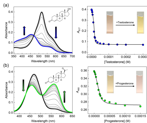
Fig. 2 UV-vis absorption spectra of the complex of indicator (10 \mu\text{M} ) and CB[8] (20 \mu\text{M} ) upon the addition of target steroid hormones in an aqueous DMSO solution (DMSO:water = 1:9, v/v) at pH 3.2 at 25 ^{\circ}\text{C} . (a) 2 for testosterone and (b) 3 for progesterone. The titration isotherms were obtained by collecting the maximum absorbance at 517 nm for 2 and 460 nm for 3 . Insets show color changes in chemosensors before and after adding (a) testosterone (300 \mu\text{M} ) and (b) progesterone (150 \mu\text{M} ), respectively. [Indicator] = 10 \mu\text{M} , [CB[8]] = 20 \mu\text{M} .
