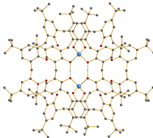
Fig. 6 The structure of the anion of compound 14 . Colour code: Co = sky blue, O = red, C = grey, H = white. The \text{Co}-\text{O}-\text{H} \cdots \text{O}-\text{Co} H-bonds are shown by the dashed black lines. These H atoms are included, while all others are omitted for clarity.
