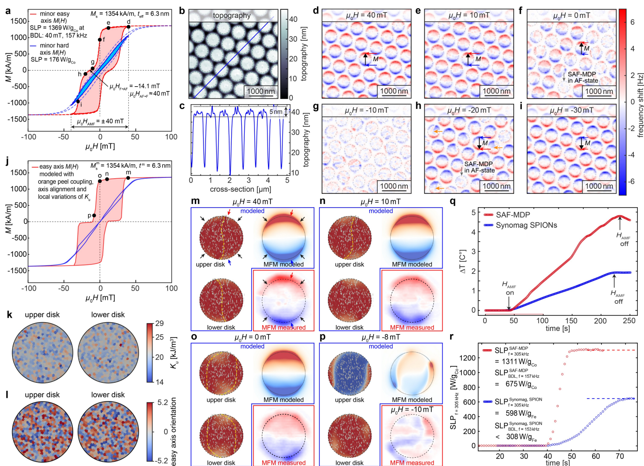
FIG. 3: SAF-MDP magnetic and hyperthermia characterization. a VSM measurements of the easy axis M(H) -loop (solid and dashed red curves, for the minor and major loop, respectively), hard axis M(H) -loop (solid and dashed blue curves, for the minor and major loop, respectively) of our SAF-MDPs still attached to the wafer ( D = 500 nm, 7 nm-thick \text{Co}_{97}\text{Sm}_3 F layers separated by 2 nm of \text{Al}_{70}\text{Zr}_{30} ). The labels d to i refer to the corresponding MFM data displayed in panels d to i . b topography image and c cross-section of the SAF-MDP islands. d to i magnetization reversal of the SAF-MDP studied by magnetic force microscopy (MFM) performed in fields applied along the easy axis, ranging from 40 mT to -30 mT. j easy and hard axis (red and blue lines, respectively) M(H) -loops obtained from a refined micromagnetic model using distinct distributions anisotropies and easy axes alignments of the grains in the upper and lower disks as displayed in k and l , respectively, and employing a roughness-induced ferromagnetic orange-peel coupling between the FLs. m to p show magnetic moment distributions of the upper and lower disk of a SAF MDP (top left and bottom left), MFM patterns calculated from these (top right) and experimental MFM data (bottom right) for 40, 10, 0, and -8 mT applied fields. q temperature rise as a function of time for suspensions of 80 \mu\text{g}_{\text{Co,Fe}}/\text{ml} of SAF-MDP and Synomag superparamagnetic nanoparticles. r evolution of the SLP values with time for suspensions of the AF-MDP and Synomag superparamagnetic nanoparticles calculated from q .
