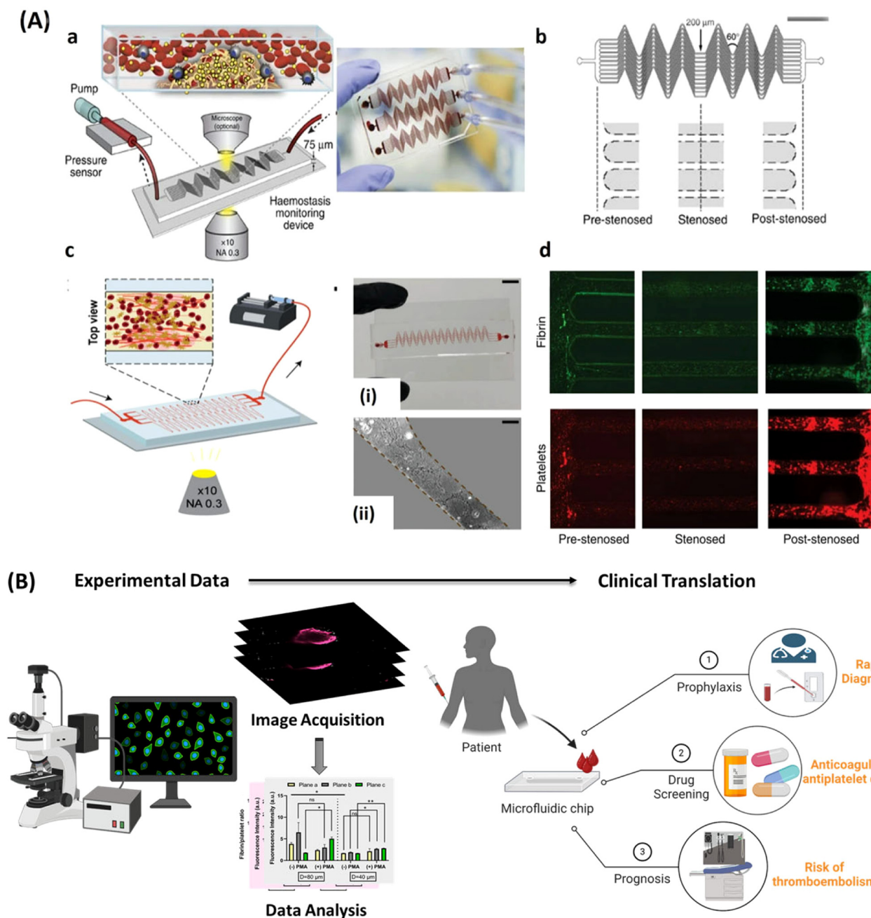
Fig. 6 (A) Microfluidic devices for haemostasis and thrombosis research. (a) Schematic of the haemostasis monitor devices and blood perfusion. Human whole blood is pushed or pulled by a syringe pump that connects to the device via tubing to determine micro-clotting time. (b) Diagram of the device with line drawings illustrating the design of the accelerating (pre-stenosed), uniform width (stenosed) and decelerating (post-stenosed) regions of the microchannels. The central stenosed region contains 12 parallel lanes of 200 \mu\text{m} -wide and 75 \mu\text{m} -high channels that repeatedly turn 60° a few times in each channel (scale: 500 \mu\text{m} ). 100 (c) Schematic of the microfluidic device mounted on a microscope and connected to a pump that pulls blood to determine clotting time, (c-i) Photograph of the microfluidic device (scale: 10 mm), (c-ii) Representative image of collagen coating a section of the microdevice (scale: 100 \mu\text{m} ). 101 (d) Fluorescence microscopy of fibrin (green) and platelets (red) in monitoring of thrombus formation in pre-stenosed, stenosed, and post-stenosed regions after perfusing blood through the device, containing heparin (0.25 IU \text{mL}^{-1} ) for 20 min (scale: 500 \mu\text{m} ). 100 (B) Translating experimental data to clinical applications in bench-to-bed side thrombosis management. Figures created with BioRender.com.
