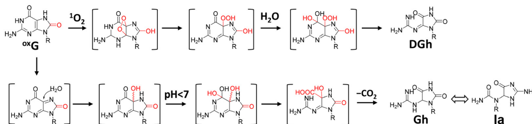
Scheme 1 Proposed mechanism for the production of the oxidized species of ox G, Gh/Ia and DGh, in 5'-Cp ox G by 1 O 2 during the photodecomposition of complex 1 upon blue light irradiation for 1 h (the bound Pt units are omitted for clarity).
