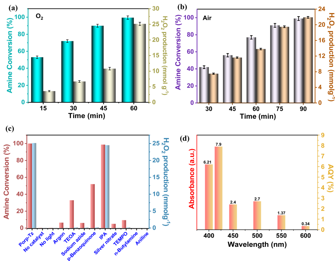
Fig. 3 (a) Time-dependent amine conversion and \text{H}_2\text{O}_2 in \text{O}_2 ; (b) time-dependent amine conversion and \text{H}_2\text{O}_2 production in air; (c) controlled experiments (TEOA – hole scavenger, sodium azide-singlet oxygen quencher, p-benzoquinone-superoxide quencher, IPA-hydroxyl radical scavenger, and silver nitrate-electron scavenger); and (d) apparent quantum yield of Porp-Tz at different wavelengths.
