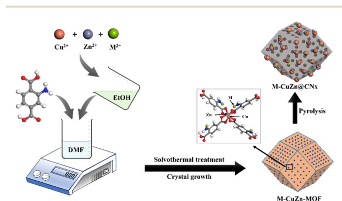
Fig. 1 Schematic representation of the synthesis procedure of M-CZ@CNx catalysts.
