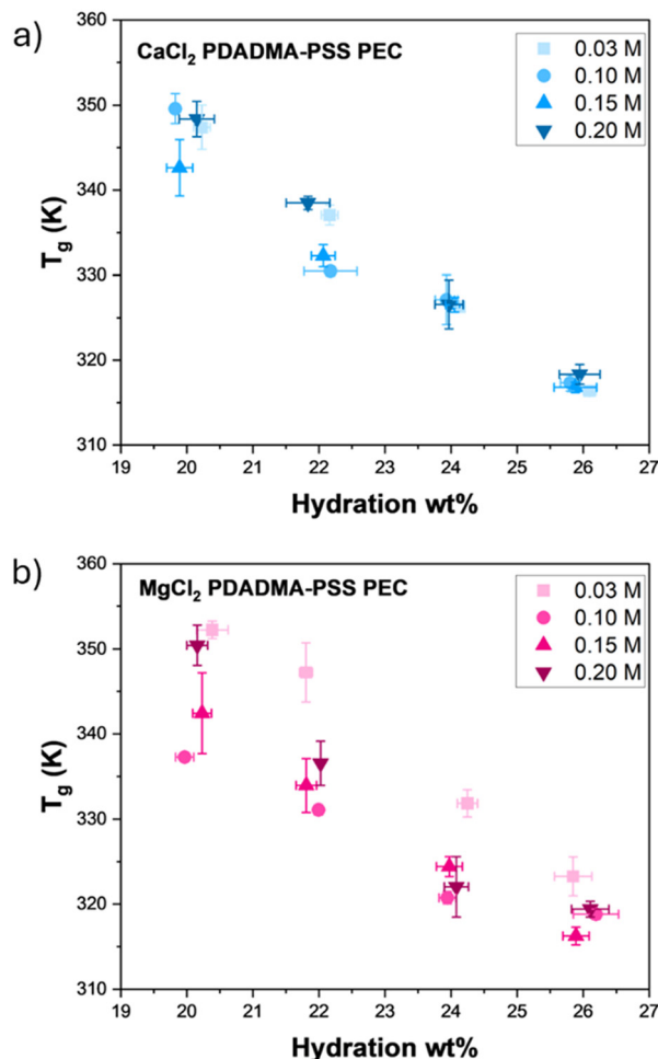
Fig. 5 Glass transition temperatures of PDADMA-PSS PECs prepared from solutions of varying (a) \text{CaCl}_2 or (b) \text{MgCl}_2 concentrations (0.03–0.20 M). The isolated PECs were rehydrated with a solution matching that of its assembly and examined using MDSC.
