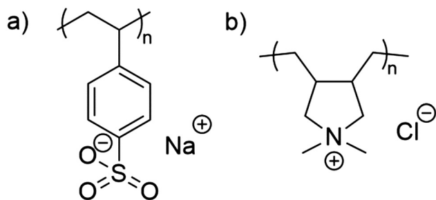
Fig. 1 Structures of polyelectrolytes used in this study. (a) Poly(styrene sulfonate) (PSS) and (b) poly(diallyldimethylammonium) (PDADMA).
