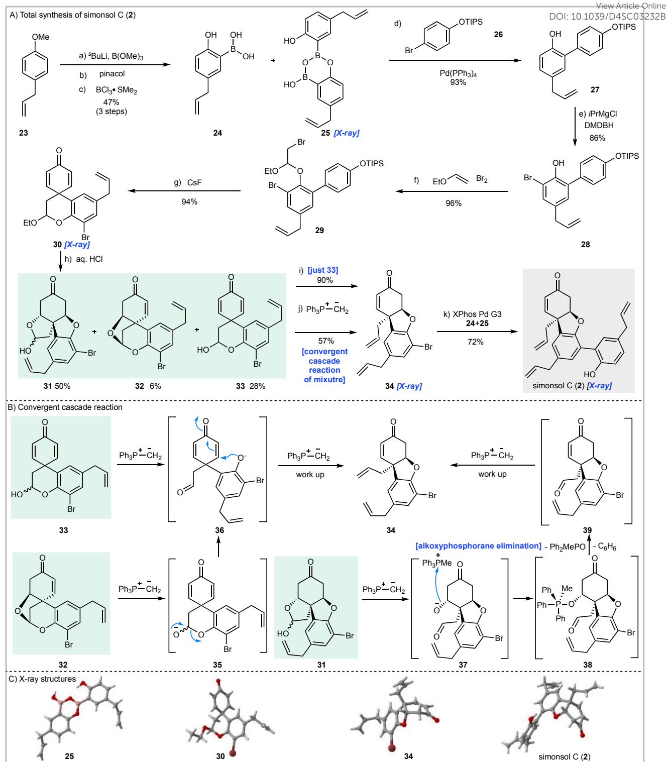
Scheme 2. Total synthesis of simonsol C (2). a Reagents and conditions: (a) s\text{BuLi} , \text{B}(\text{OMe})_3 , \text{TMEDA} , \text{THF} , -78^\circ\text{C} to r.t., 1 h; (b) pinacol, methanol, r.t., 16 h; (c) \text{BCl}_3 \cdot \text{SMe}_2 , 1,2-DCE, 80^\circ\text{C} , 16 h, 47% (3 steps); (d) \text{Pd}(\text{PPh}_3)_4 (8 mol%), aq. \text{Na}_2\text{CO}_3 , \text{THF} , r.t. 1.5 h, 93%; (e) \text{DBDMH} , i\text{PrMgCl} , \text{THF} , -78^\circ\text{C} to r.t., 1.5 h, 86%; (f) ethyl vinyl ether, \text{Br}_2 , Hünig's base, \text{DCM} , 0^\circ\text{C} to r.t., 2.5 h, 96%; (g) \text{CsF} , \text{Na}_2\text{SO}_4 , \text{DMF} , 130^\circ\text{C} , 1 h, 94%; (h) \text{HCl} aq., 1,4-dioxane, 80^\circ\text{C} , 10.5 h, 33 28%, 32 6%, 31 50%; (i) \text{MePPh}_3 \text{Br} , \text{KHMDS} , \text{THF} , 0^\circ\text{C} , 1 h, 90% (just 33 ); (j) \text{MePPh}_3\text{Br} , \text{KHMDS} , \text{THF} , 0^\circ\text{C} , 1 h, 57% (convergent cascade reaction of mixture); (k) \text{XPhos Pd G3} 10 mol%, aq. \text{K}_3\text{PO}_4 , \text{THF} , 50^\circ\text{C} , 1.3 h, 72%. \text{THF} = tetrahydrofuran, \text{TMEDA} = N,N,N',N' -tetramethylethylenediamine, \text{DBDMH} = dibromo dimethyl hydantoin, \text{DMF} = dimethylformamide, \text{KHMDS} = potassium hexamethyldisilazide
