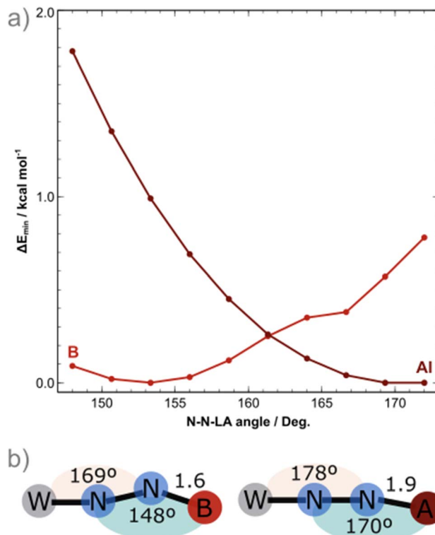
Fig. 2 (a) Potential energy surface along the N–N–Lewis acid angle coordinate for the AICF (crimson) and BCF (red) 1 : 1 adducts, energies reported relative to PES minimum; and (b) relevant angles of the optimized structures.
