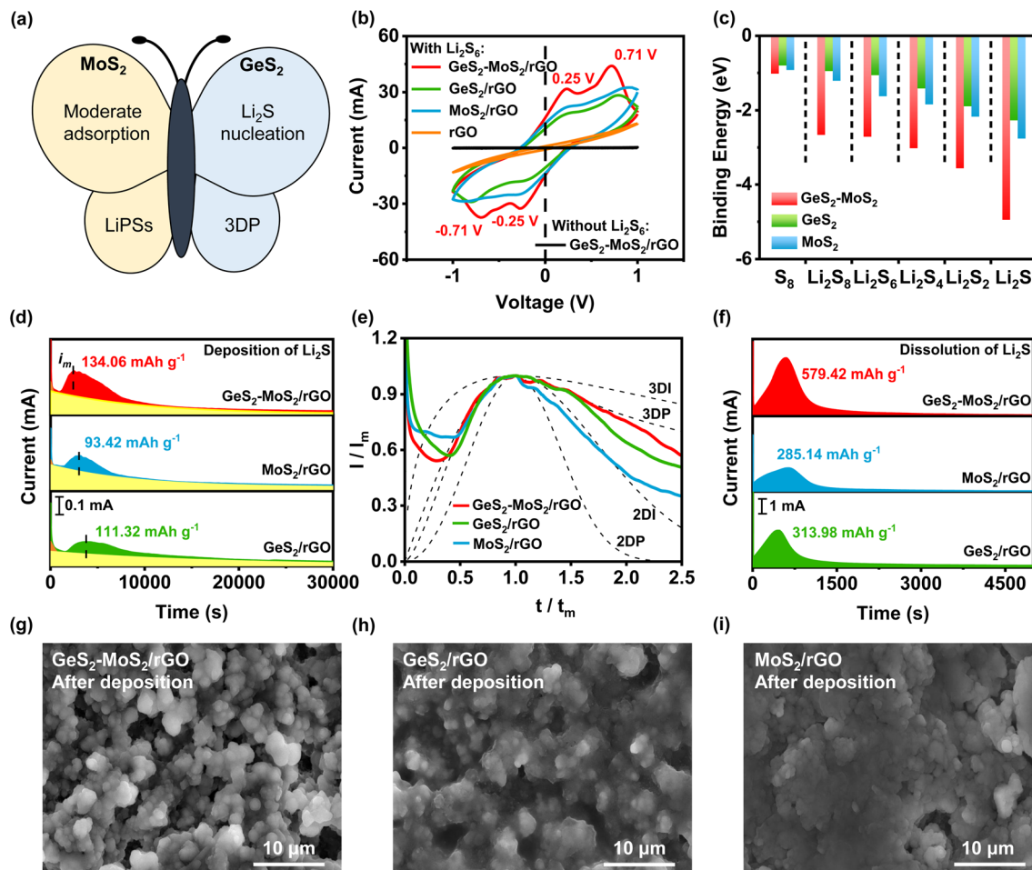
Fig. 4 (a) Schematic illustration of the \text{GeS}_2 - \text{MoS}_2 heterostructure. The butterfly heterostructure is designed as a sulfur host to facilitate the conversion of LiPSs and promote the growth of \text{Li}_2\text{S} synergistically. (b) CV curves of different catalysts in symmetric batteries at a scan rate of 20 \text{ mV s}^{-1} . \text{GeS}_2 - \text{MoS}_2/\text{rGO} has the strongest peak current density and the smallest overpotential; (c) binding energies of \text{S}_8 and \text{Li}_2\text{S}_x ( x = 1, 2, 4, 6, \text{ and } 8 ) species on different catalysts. The \text{GeS}_2 - \text{MoS}_2 heterostructure has the strongest binding energy with LiPSs, effectively promoting the catalytic effect. (d) Potentiostatic discharge profiles at 2.05 \text{ V} with \text{Li}_2\text{S}_8 catholyte on different samples. The \text{GeS}_2 - \text{MoS}_2/\text{rGO} heterostructure with rich catalytic heterointerfaces can achieve rapid conversion of LiPSs and advanced deposition of \text{Li}_2\text{S} . (e) Dimensionless transient (symbols) of different samples in comparison with theoretical 2D and 3D models ( I_m : peak current; t_m : time needed to achieve the peak current). \text{Li}_2\text{S} growth follows a typical 3DP mode in the \text{GeS}_2 - \text{MoS}_2/\text{rGO} heterostructure. (f) Potentiostatic charge profiles of different samples at 2.40 \text{ V} for \text{Li}_2\text{S} dissolution. (g–i) SEM images of \text{GeS}_2 - \text{MoS}_2/\text{rGO} , \text{GeS}_2/\text{rGO} and \text{MoS}_2/\text{rGO} after \text{Li}_2\text{S} deposition. The uniform and radial deposition of \text{Li}_2\text{S} is achieved on the surface of the \text{GeS}_2 - \text{MoS}_2/\text{rGO} heterostructure.
