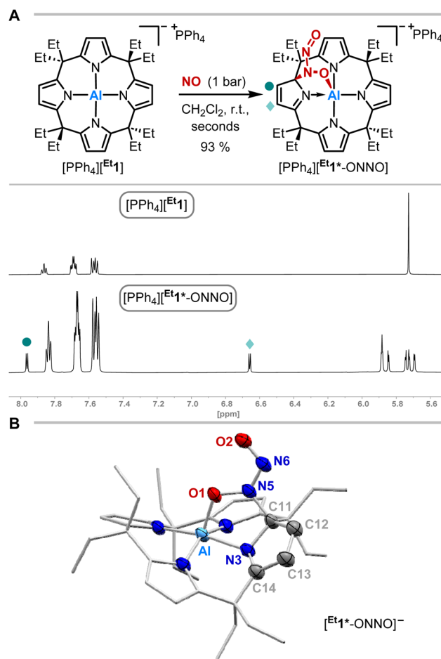
Fig. 2 (A) Synthetic scheme for the reaction of [PPh 4 ][ E1 ] with nitrogen monoxide and excerpts of the 1 H NMR spectra (600 MHz, CD 2 Cl 2 ) of [PPh 4 ][ E1 ] (top) and [PPh 4 ][ E1 *-ONNO] (bottom). (B) Solid state molecular structure of [ E1 *-ONNO] – as determined by SCXRD analysis. The tetraphenylphosphonium counterion, cocrystallized solvent molecules, and all hydrogen atoms are omitted for clarity. Thermal displacement ellipsoids are displayed at the 50% probability level. Selected bond lengths [pm]: Al–O1: 185.0(2), O1–N5: 135.9(3), N5–N6: 130.1(3), N6–O2: 123.3(3), N5–C11: 149.4(4), N3–C11: 146.4(3), C11–C12: 150.6(4), C12–C13: 133.0(4), C13–C14: 147.4(4), C14–N3: 128.3(4), N3–C11: 146.4(3), Al–N3: 199.7(3). Selected bond angles [°]: Al–O1–N5: 112.52(17), O1–N5–N6: 123.1(3), N5–N6–O2: 115.7(2). Selected dihedral angle [°]: O1–N5–N6–O2: 1.8(4).
