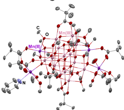
Fig. 1 Solid state structures of [\text{Mn}_{18}\text{-Ac}] (a) and [\text{Mn}_{18}\text{-Piv}] (b) drawn with thermal ellipsoids at the 30% probability level. Hydrogen atoms are omitted for clarity. Colour code: Mn II , purple; Mn III , pink; O, red; N, blue; C, grey.
