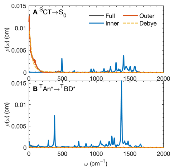
Fig. 4 Spectral distribution \rho(\omega) for (A) the S^{\text{CT}} \rightarrow S_0 process computed from dynamics on the S^{\text{CT}} potential energy surface and (B) the T^{\text{An}^*} \rightarrow T^{\text{BD}^*} process computed from dynamics on the T^{\text{An}^*} potential energy surface. The decomposition into inner and outer sphere contributions and the Debye approximation for the outer-sphere component is also shown, \rho_D(\omega) = (2/\pi)/(1 + \tau_D^2\omega^2) , where \tau_D = (\epsilon_\infty/\epsilon_r)\tau_{\text{rel}} , and \tau_{\text{rel}} is the solvent dipole-dipole autocorrelation relaxation time, and \epsilon_\infty/\epsilon_r are the optical and static dielectric constants of the ACN model.
