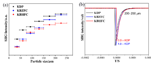
Fig. 3 (a) Powder SHG measurements of KDP, KBZFC, and KBHFC at 1064\text{ nm} . (b) SHG signals from KBZFC and KBHFC compared with benchmark KDP at 200\text{--}250\text{ }\mu\text{m} .
