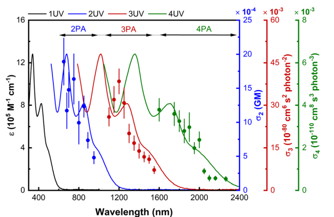
Fig. 3 Wavelength dependence of the nonlinear absorption of 3G 22,03,02,01 -NO 2 . Plots of \sigma_2 (blue scatter), \sigma_3 (red scatter), and \sigma_4 (green scatter), overlaid on the UV/Vis spectrum (black line), and including plots of the UV/Vis spectrum as a function of twice (blue line), three times (red line), and four times (green line) the wavelength.
