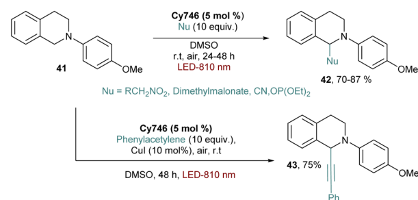
b) \alpha -nitrogen radical
