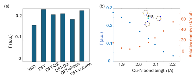
Fig. 9 (a) The EFG distance of optimized \text{Cu}_3(4\text{hypycca})_3 structure with different approaches, along with (b) the dependence of \Gamma on Cu-N bond length.
