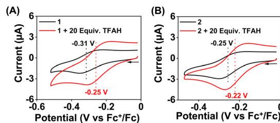
Fig. 5 Cyclic voltammogram of 1 (0.5 mM) (A) and 2 (0.5 mM) (B) in the presence and absence of excess TFAH (10 mM) in acetonitrile containing n Bu 4 NPF 6 (50 mM) as the supporting electrolyte under a N 2 atmosphere (scan rate 0.1 V s –1 ). A 3 mm glassy carbon working electrode and Pt wire counter electrode were used during the measurements.
