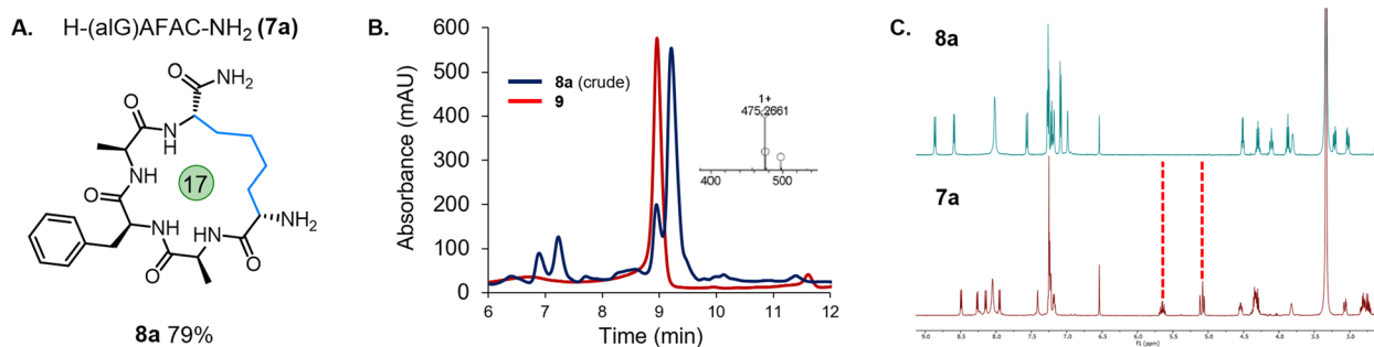
Fig. 2 (A) Cyclised peptide 8a from H-(alG)AFAC-NH 2 ( 7a ); (B) analytical HPLC of the crude cyclisation of 7a (blue trace) overlaid with peptide H-(alG)AFAC-NH 2 ( 9 ), inset – ESI MS showing the mass of the desired cyclised product ( 8a ); (C) 1 H NMR spectrum for linear peptide 7a (red trace) and peptide macrocycle 8a (blue trace) showing the absence of the allylic protons.
