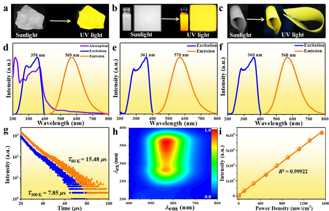
Fig. 2 PL characterization of (Im-BDMPA) \text{In}_{0.78}\text{Sb}_{0.22}\text{Cl}_6 \cdot \text{H}_2\text{O} : (a–c) photo images of bulk crystals, microparticles, the deposited thin film and the flexible composite film under sunlight and 365 nm UV light; (d–f) absorption, excitation and emission spectra of bulk crystals, microparticles and flexible composite; (g) PL decay curves at 300 K and 80 K; (h) 3D consecutive PL map; (i) power density dependent PL emission intensity.
