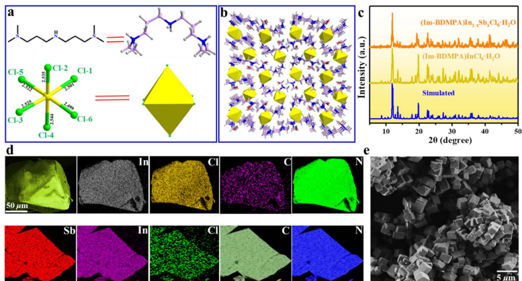
Fig. 1 Structural characterization of (Im-BDMPA) \text{In}_{1-x}\text{Sb}_x\text{Cl}_6 \cdot \text{H}_2\text{O} : (a) (Im-BDMPA) ^{3+} cation and [\text{In}/\text{SbCl}_6]^{3-} octahedron; (b) packing structure of the OD structure viewed along the a -axis; (c) simulated and experimental PXRD patterns; (d) elemental mapping of SEM images; (e) SEM image of a microparticle.
