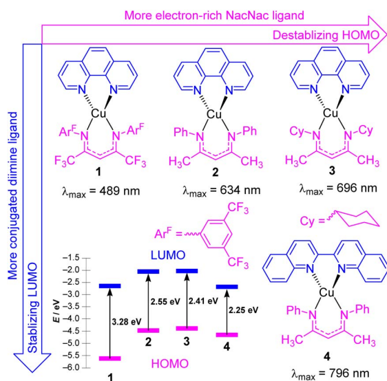
Fig. 2 Summary of heteroleptic \text{Cu}(\text{NacNac}^R) complexes and their frontier orbital energy levels. Frontier orbital energies were determined by DFT.
