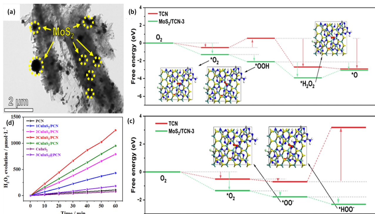
Fig. 27 (a) SEM images of MoS 2 -TCN-3. Free energy change graphs for the \text{O}_2 reduction reaction ( 2\text{e}^- ORR) under (b) acidic and (c) alkaline conditions. The figures are adapted with permission from ref. 201. Copyright 2023, Elsevier. (d) Photocatalytic \text{H}_2\text{O}_2 generation by PCN, CuInS 2 , 3CuInS 2 @PCN, and xCuInS 2 /PCN samples. The figures are adapted with permission from ref. 202. Copyright 2023, Elsevier.
