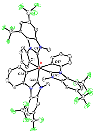
Fig. 1 Structure drawing of m\text{-Ir}(\text{dfp})_3 with thermal ellipsoids shown at the 30% probability level. Selected bond length (Å): Ir–C1 = 2.076(3), Ir–C7 = 2.006(3), Ir–C17 = 2.112(3), Ir–C23 = 2.047(3), Ir–C33 = 2.104(3), and Ir–C39 = 2.021(3). Selected bond angle (°): C1–Ir–C23 = 169.91(10), C7–Ir–C39 = 166.42(10), and C17–Ir–C33 = 177.97(11).
