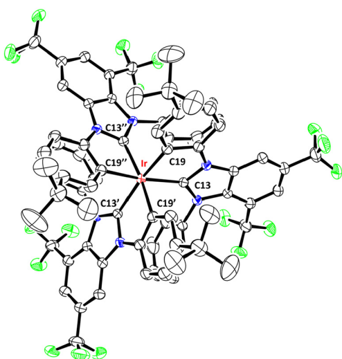
Fig. 2 Structure drawing of f\text{-Ir}(\text{tBpp})_3 with thermal ellipsoids shown at the 30% probability level. Selected bond length (Å): Ir–C13 = 2.0428(17) and Ir–C19 = 2.0903(19). Selected bond angles (°): C13–Ir–C19' = 168.52(8).
