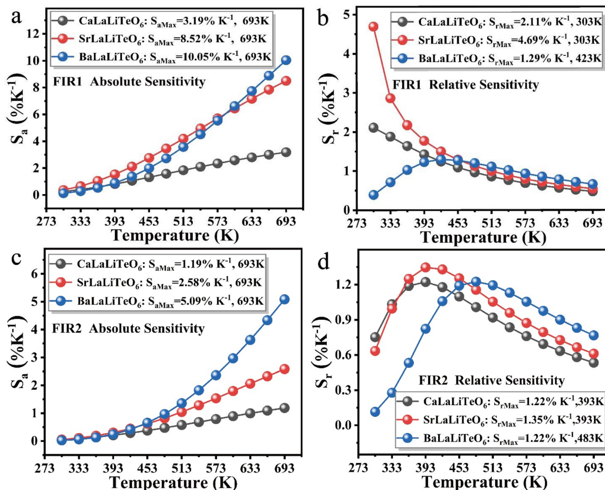
Fig. 7 (a and b) The calculated S_a and S_r values of \text{ALaLiTeO}_6:\text{Yb}^{3+},\text{Tm}^{3+} based on FIR 1 . (c and d) The calculated S_a and S_r values of \text{ALaLiTeO}_6:\text{Yb}^{3+},\text{Tm}^{3+} based on FIR 2 .
