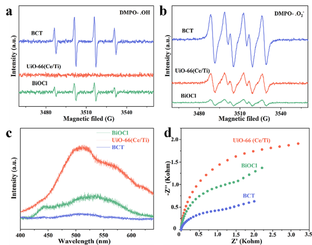
Fig. 6 Electron paramagnetic resonance (EPR) spectra of (a) DMPO–OH adducts and (b) DMPO–O 2 •− adducts over BiOCl, UiO-66(Ce/Ti), and BCT under illumination for 2 min. (c) Steady-state photoluminescence (PL) spectra and (d) electrochemical impedance spectroscopy (EIS) spectra of BiOCl, UiO-66(Ce/Ti), and BCT.
