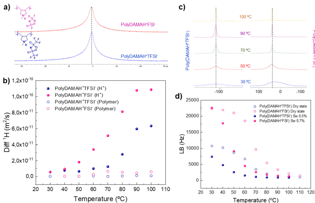
Fig. 1 ^1\text{H} SPE NMR spectra for poly(DAMAH + TFSI - ) and poly(DAMAH + FSI - ) at 110 °C in the dry state (a); diffusion coefficients of both protic poly(ionic liquids) by ^1\text{H} PFG NMR obtained under 75 RH% from 30 to 100 °C (b); ^{19}\text{F} SPE NMR spectra of both protic poly(ionic liquids) under 75 RH% from 30 to 100 °C (c); and line broadening (LB) comparison between dry and swelled states (d).
