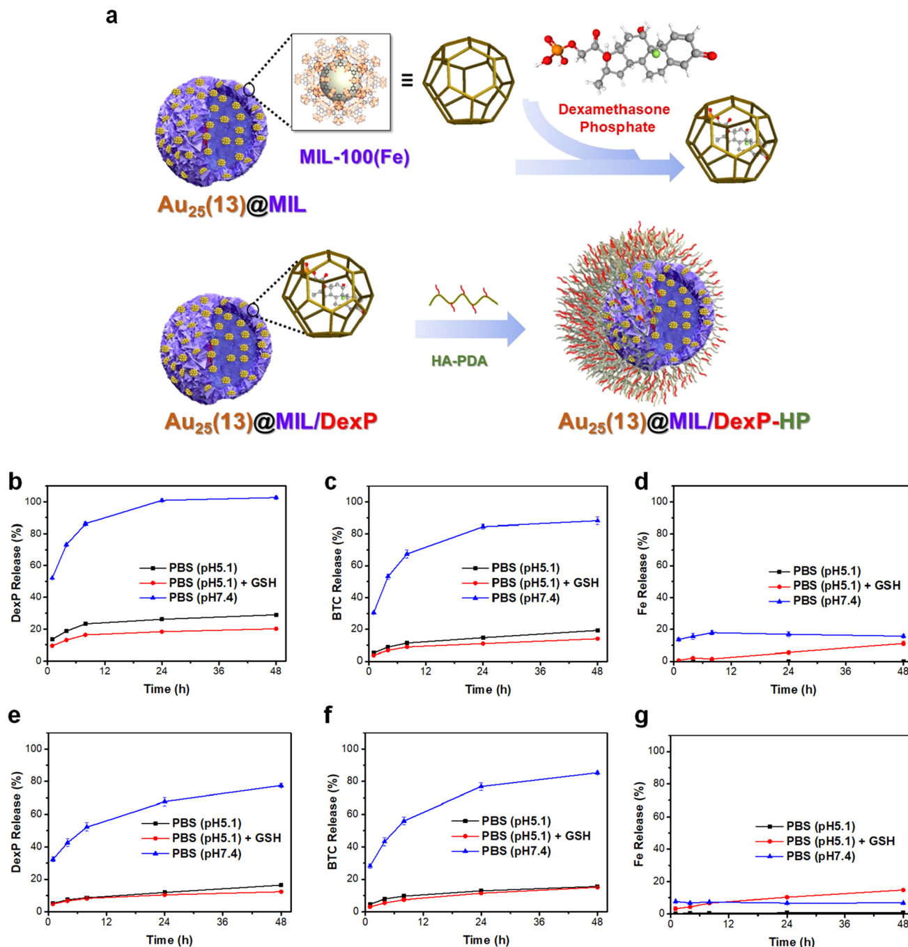
Fig. 3 (a) Scheme of the DexP loading in \text{Au}_{25}(\text{13})@\text{MIL} and its surface functionalization by HA-PDA; (b and e) DexP, (c and f) BTC and (d and g) Fe release from (b–d) \text{Au}_{25}(\text{13})@\text{MIL}/\text{DexP} and (e–g) \text{Au}_{25}(\text{13})@\text{MIL}/\text{DexP-HP} in different PBS media (i.e. PBS at pH 5.1, PBS at pH 5.1 with 10 mM GSH and PBS at pH 7.4). The DexP and BTC releases were measured by HPLC and the Fe release by ICP-MS. The experiments were performed in triplicate.
