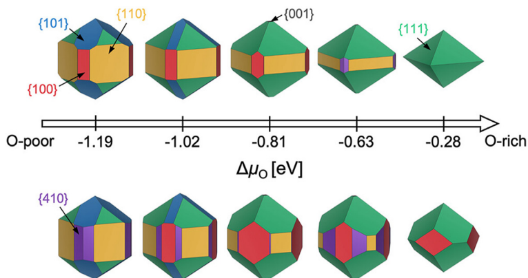
Fig. 3 Equilibrium Wulff nanoparticle shapes computed from \text{RuO}_2 surface energies of all low-index (up to (111)) facets and the (410) vicinal, using locally optimized structures (top) and global geometry optimized structures (bottom). The indicated changes in oxygen chemical potential, \Delta\mu_{\text{O}} , correspond to calcination pretreatment conditions used by Rosenthal et al. , 30,31 Jirkovský et al. , 32 Lee et al. , 33 and Narkhede et al. , 34 from left to right. Standard conditions (300 K, 1 bar, -0.28 eV) are also displayed. This figure has been reproduced from ref. 26 with permission from the American Chemical Society, copyright 2023.
