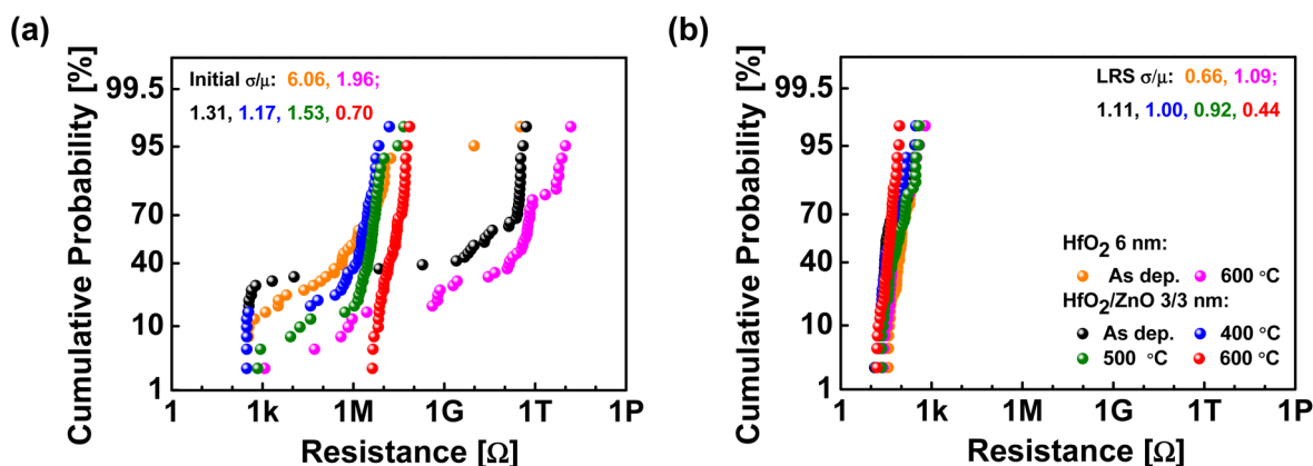
Fig. 4 Distribution and cumulative probability of (a) the initial state during the electroforming process and (b) the low-resistance state (LRS) for single-layer \text{HfO}_2 and bilayer \text{HfO}_2/\text{ZnO} synaptic devices without and with thermal annealing, where the initial state and LRS were extracted at a read voltage of \pm 0.3 V.
