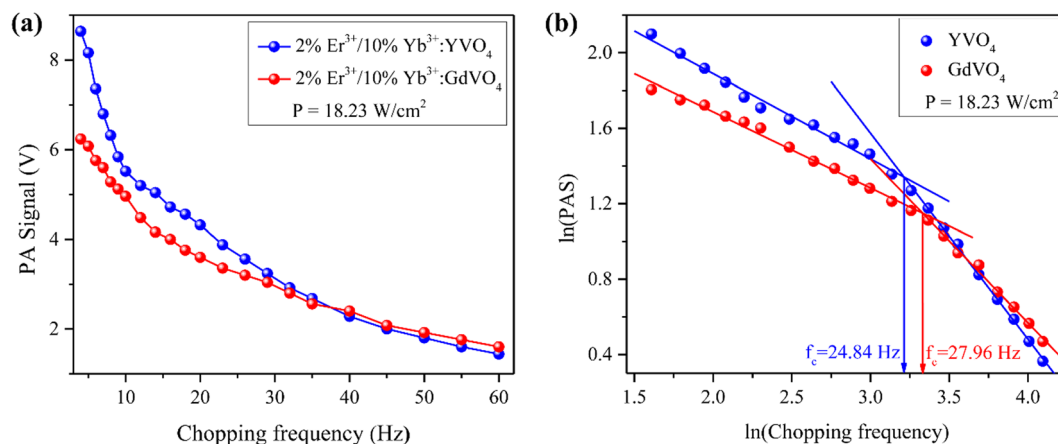
Fig. 9 (a) Variation of the photoacoustic signal amplitude with chopping frequency at an excitation power density of 18.23 W cm −2 and (b) \ln(\text{chopping frequency}) – \ln(\text{PAS}) graph for transition frequency calculation.
