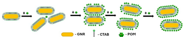
Scheme 2 Formation of the GNR-CTAB-POM1 structure. At low POM1 concentration the POM1 leads to unstable aggregation of GNRs. Higher POM1 concentration leads to stable aggregates, then no GNR aggregation and finally full POM1 coverage of the GNRs.
