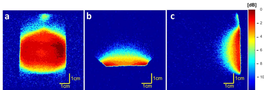
Fig. 1 Coil homogeneity measured using ^1\text{H} MRI at 4.7 T scanner in (a) coronal (b) axial and (c) sagittal planes; the color scale reflects signal attenuation (dB) – from the lowest (red) to the highest (blue).
