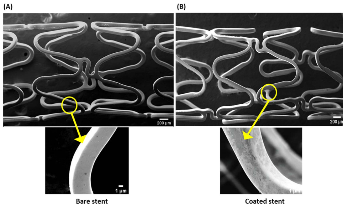
Fig. 1 Scanning electron micrographs of surface morphologies of (A) bare (uncoated) and (B) coated stents. Magnifications: upper panels, 25× (scale, 200 μm); lower panels, 400× (scale, 1 μm).
