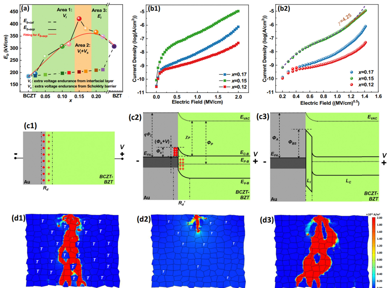
Fig. 5 (a) The variation of E_{b\text{-cal}} and E_{b\text{-exp}} with x ; the relationship between (b1) \log J and E ; (b2) \log J and E^{1/2} of BCZT- x BZT with x = 0.12 , 0.15 , and 0.17 ; (c1) the schematic illustration of the interface between the Au electrode and BCZT-0.15BZT; (c2) band diagram showing the formation of the built-in potential of BCZT-0.15BZT in a high electric field range in the \log J - E^{1/2} relationship of x = 0.15 ; (c3) the band diagram of the interface between Au electrodes and BCZT- x BZT with x = 0.12 or 0.17 ; the spread of the current density of (d1) BCZT-0.02BZT; (d2) BCZT-0.15BZT; and (d3) BCZT-0.22BZT at 400\text{ kV cm}^{-1} simulated using COMSOL Multiphysics 6.0.
