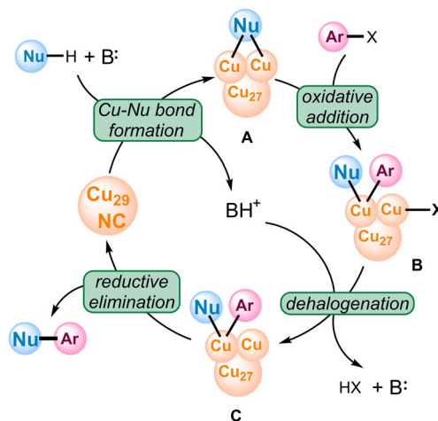
Scheme 1 Proposed catalytic cycle.
