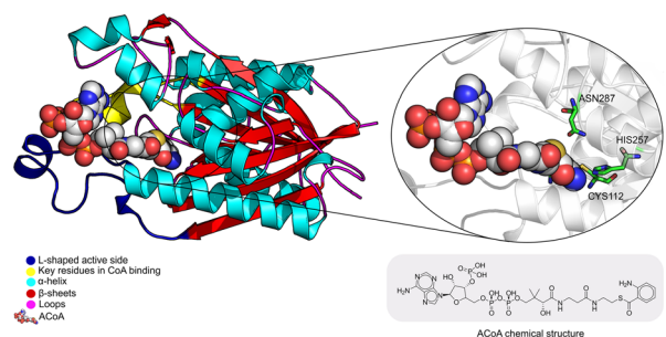
Fig. 2 Schematic representation of PqsD bound to ACoA (PDB: 3H77). Protein represented in cartoon, with key features highlighted with different colors, and ACoA represented by atom VdW radius (spheres).
